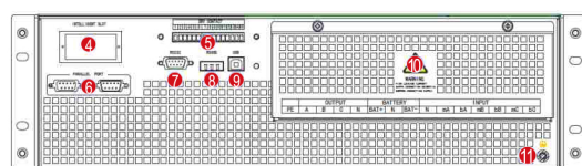
Rear panel
